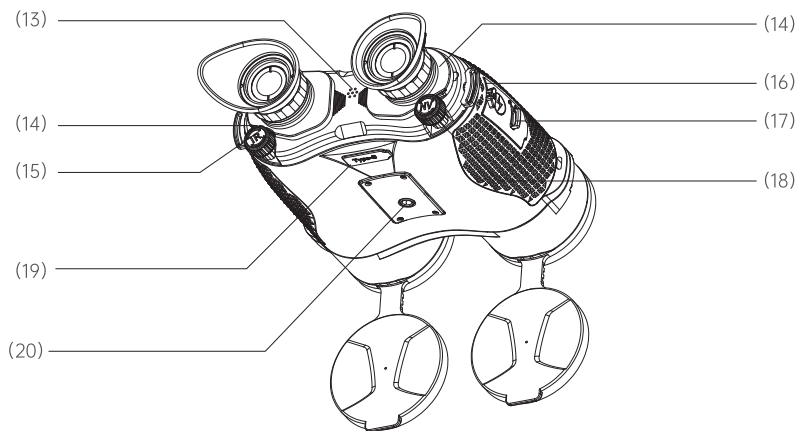
Figure 2 Rear View
