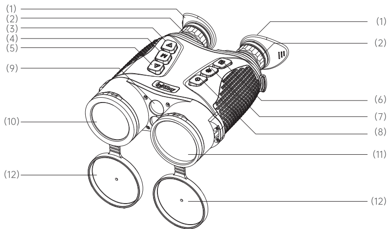
Figure 1 Front View
